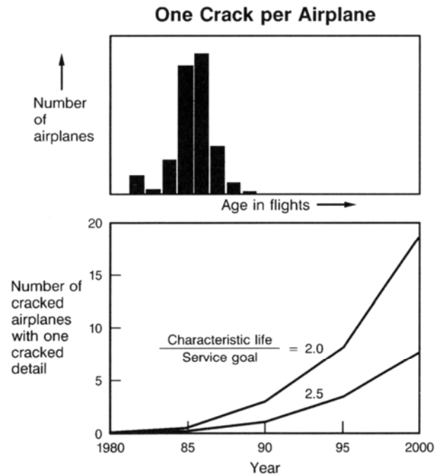
Figure 43. Predicted Fleet Cracking Example—One Crack per Airplane
