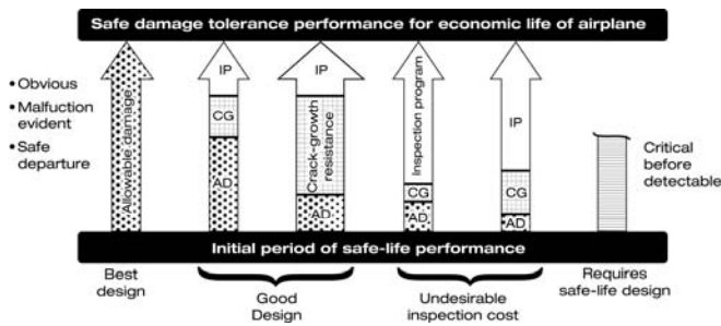
Figure 4. Interaction of Damage Tolerance Elements
