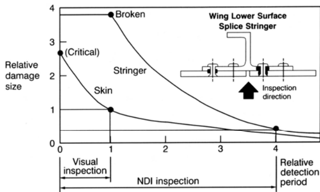
Figure 21. Visual Versus NDI Damage Detection Periods
