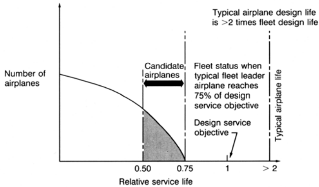
Figure 38 Supplemental Inspection Candidate Airplane Criteria
