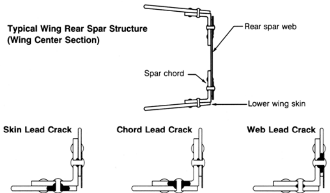
Figure 54. Wing Spar Chord Cracking Pattern Examples
