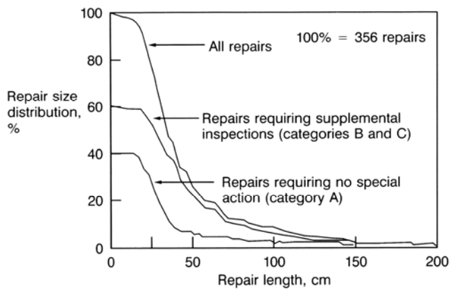
Figure 96. Fuselage Repair Size Distributions Based on Fleet Surveys
