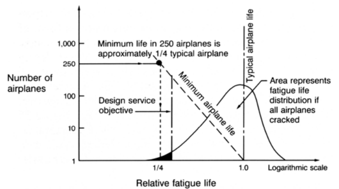
Figure 36. Variation of Minimum Life With Fleet Size
