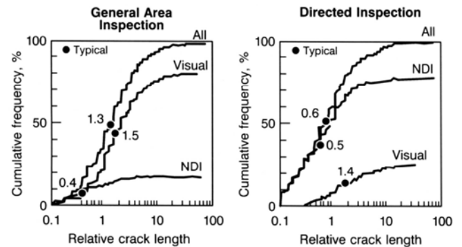
Figure 28. Distribution of Cracks Found in Service
