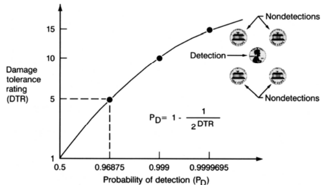
Figure 24. Probability of Detection Measurements
