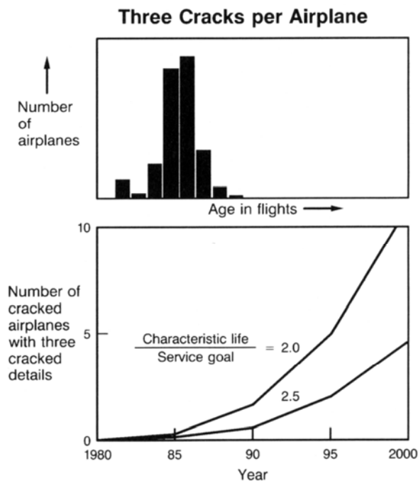
Figure 44. Predicted Fleet Cracking Example — Three Cracks per Airplane
