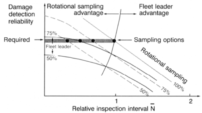
Figure 39. Fleet Sampling Options
