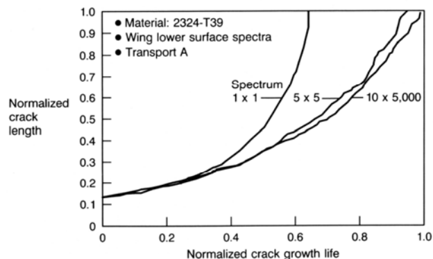
Figure 14. Effect of Spectrum Complexity on Crack Growth
