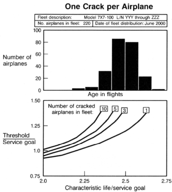
Figure 41. Fleet Service Cracking Estimate Example—One Crack per Airplane
