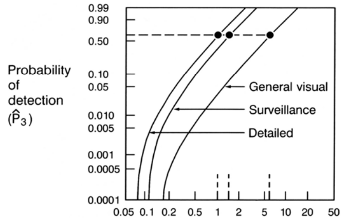
Figure 20. Relative Probability of Detection for Visual Inspection Methods
