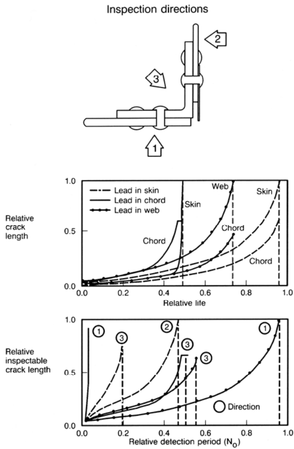
Figure 55. Spar Chord Crack Growth Curve Examples — Wing Center Section
