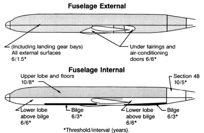
Figure 72. 727 Corrosion Control Program — Example
