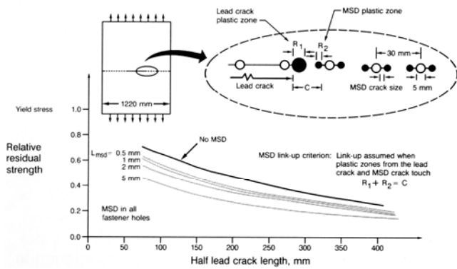
Figure 89. Residual Strength of an Unstiffened Panel Containing Various MSD Sizes
