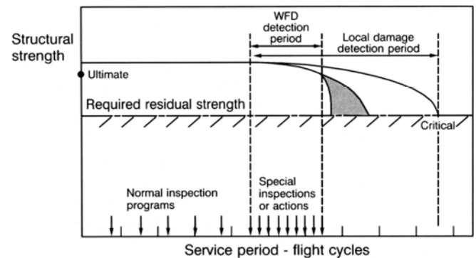
Figure 9. Damage Detection Comparisons for Local and Widespread Fatigue Damage
