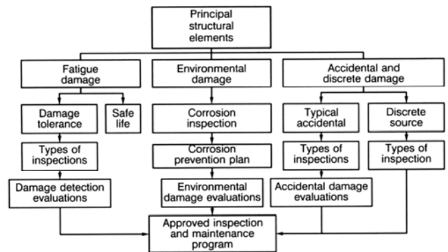
Figure 3. Principal Damage Sources for Maintenance Planning Considerations
