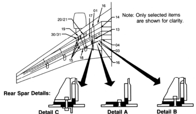
Figure 45. Structurally Significant Item Examples for Wingbox
