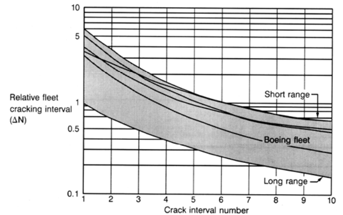
Figure 60. Fleet Cracking Variation — \Delta N
