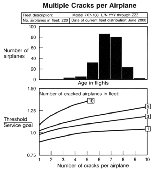
Figure 42. Fleet Service Cracking Estimate Example—Multiple Cracks per Airplane
