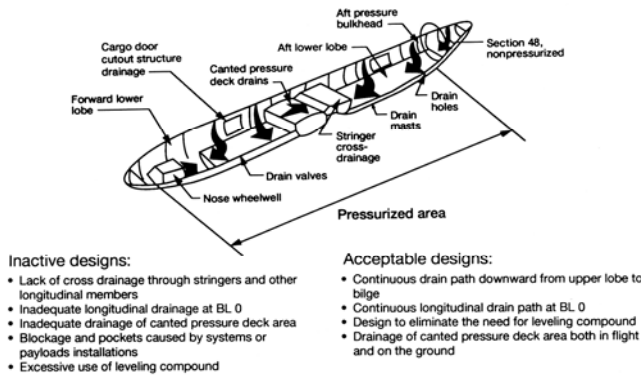
Figure 76. Lower Lobe Drainage Examples in Corrosion Prevention Design Handbook
