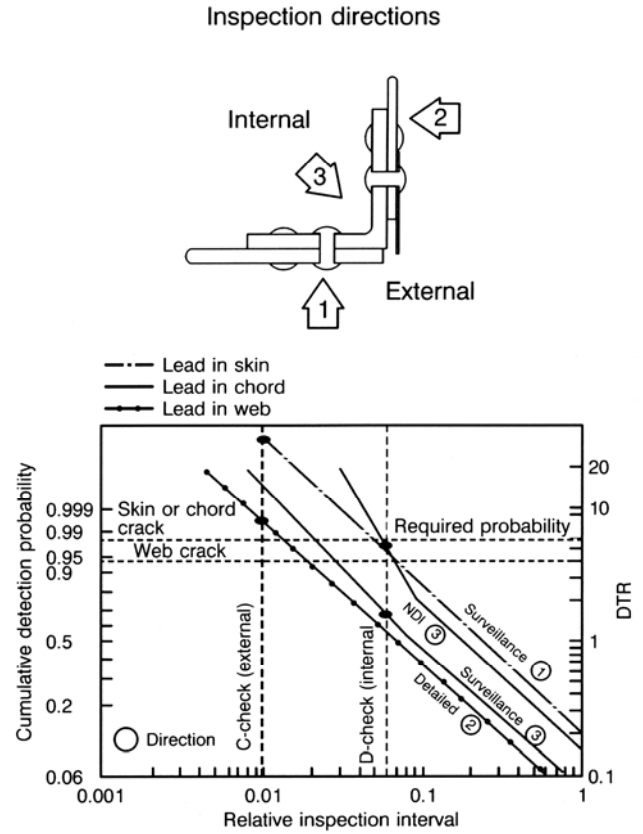
Figure 57. Cumulative Detection Probability — Cracking Pattern/Inspection Direction Combinations
