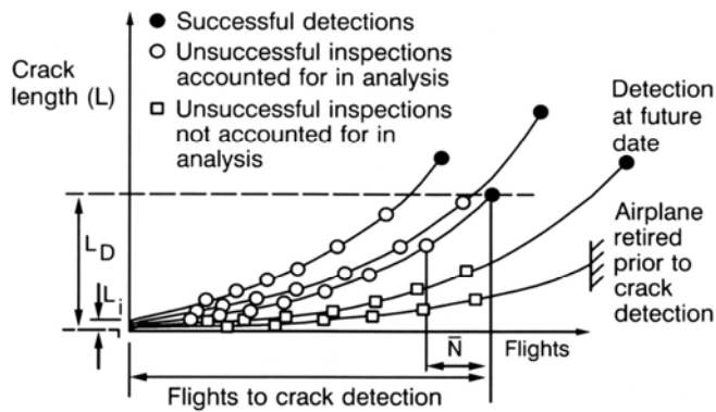
Figure 29. Detection and Nondetection Events
