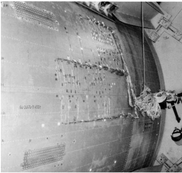
Figure 8. Typical Fuselage Pressure Test Panel
