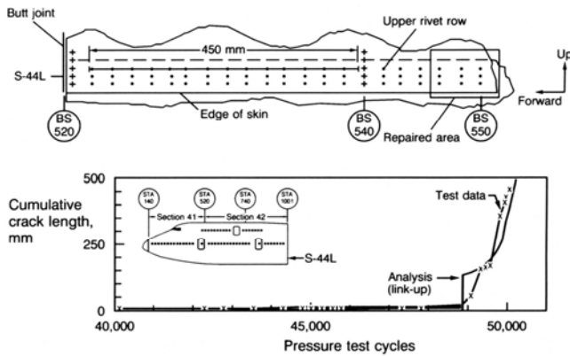
Figure 19. 747-400 Fuselage Lap Splice Test Results — Stringer 44L
