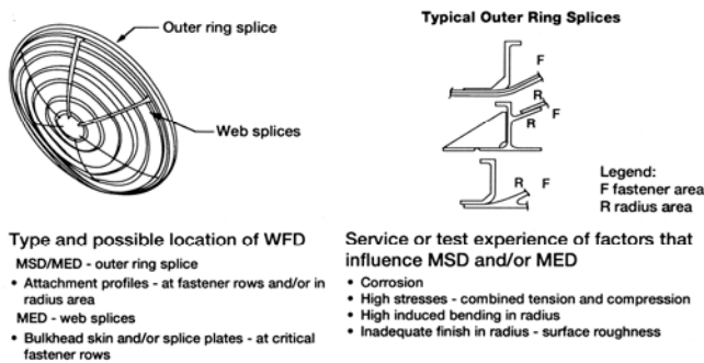
Figure 87. Structures Potentially Susceptible to WFD — Aft Pressure Dome Outer Ring and Dome Web Splices Examples
