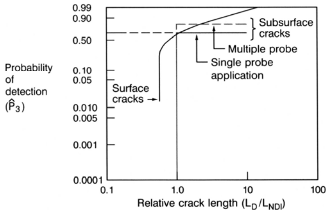
Figure 22. Probability of Detection for NDI Inspections
