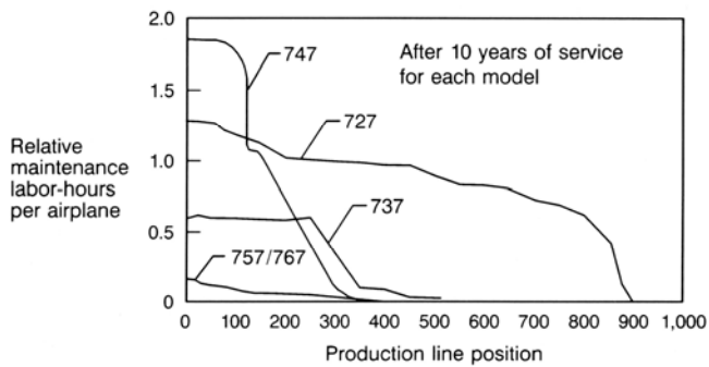
Figure 67. Comparison of Service Bulletin Labor Hours Related to Corrosion and Fatigue
