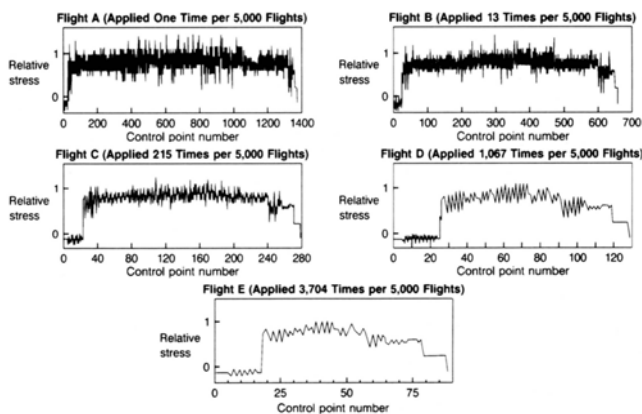
Figure 13. Wing Lower Surface Spectrum Example
