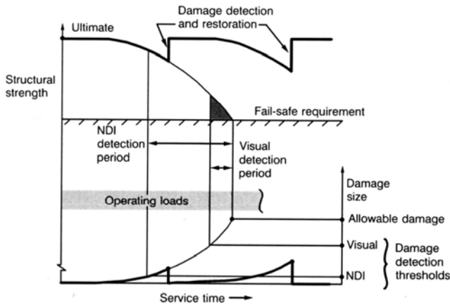
Figure 1. Strength Requirements for Damage Tolerant Structure
