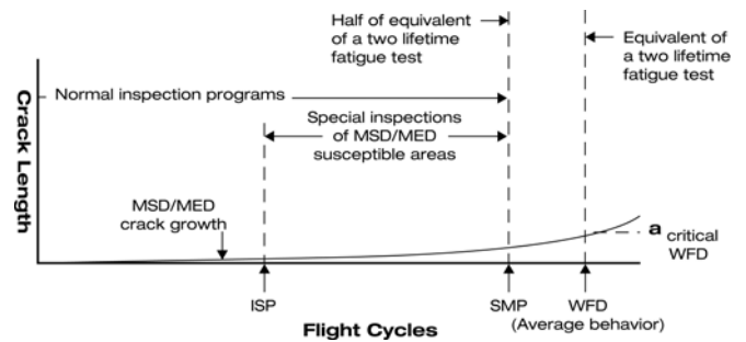
Figure 85. ISP and SMP Graphical Representation
