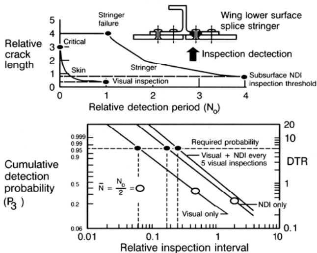
Figure 53. Cumulative Detection Probability — Inspection Method Variation
