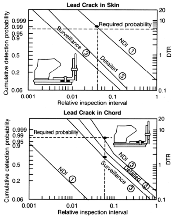
Figure 58. Cumulative Detection Probability Locally Hidden Skin Details
