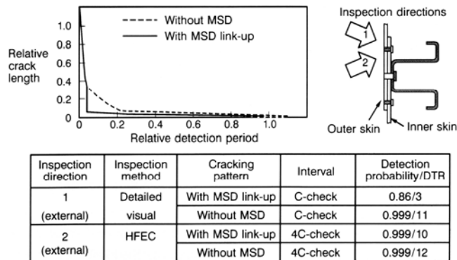
Figure 80. Example of SSID Revisions to Account for Assumed MSD Link-Up in Lap Splices
