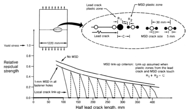
Figure 88. Residual Strength of an Unstiffened Panel Containing MSD at Each Fastener Hole
