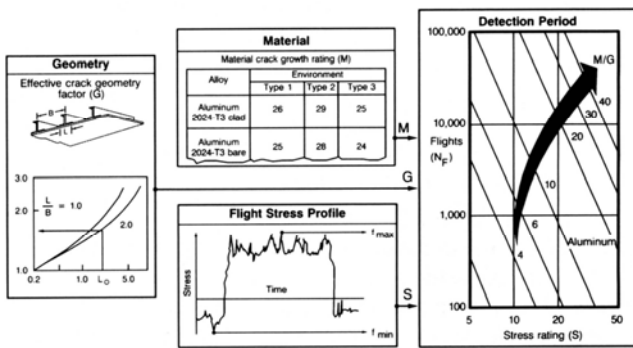
Figure 10. Crack Growth Technology Standards
