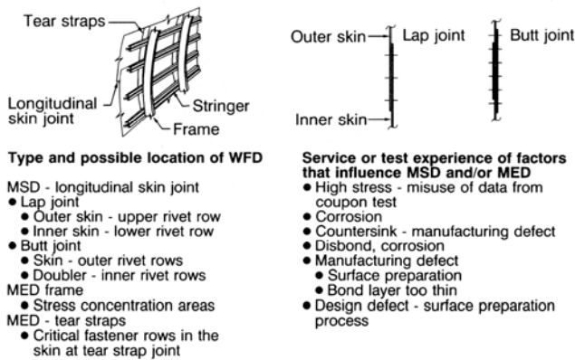
Figure 86. Structures Potentially Susceptible to WFD — Longitudinal Skin Joints, Frames and Tear Straps Examples
